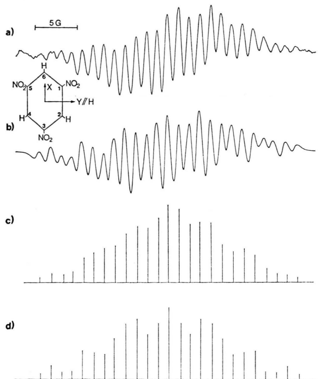
Fig. 2. Triplet-ESR-lines of the complex N-d 8 -TNB for the orientation H \parallel y , Fig. 2 a: Experimental spectrum, H_0 = 3428 \text{ G} , \nu = 9184 \text{ MHz} , T = 150 \text{ K} . Fig. 2 b: Calculated spectrum using the parameters given in the text. Figures 2 c and 2 d show the stick diagrams corresponding to the experimental and the calculated spectrum, respectively.
